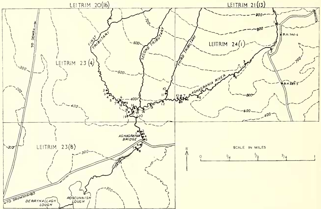
TEXT-FIG. 4. Map showing the southern area of fossiliferous localities on Slieve Anierin, including the Aghagrania River.
